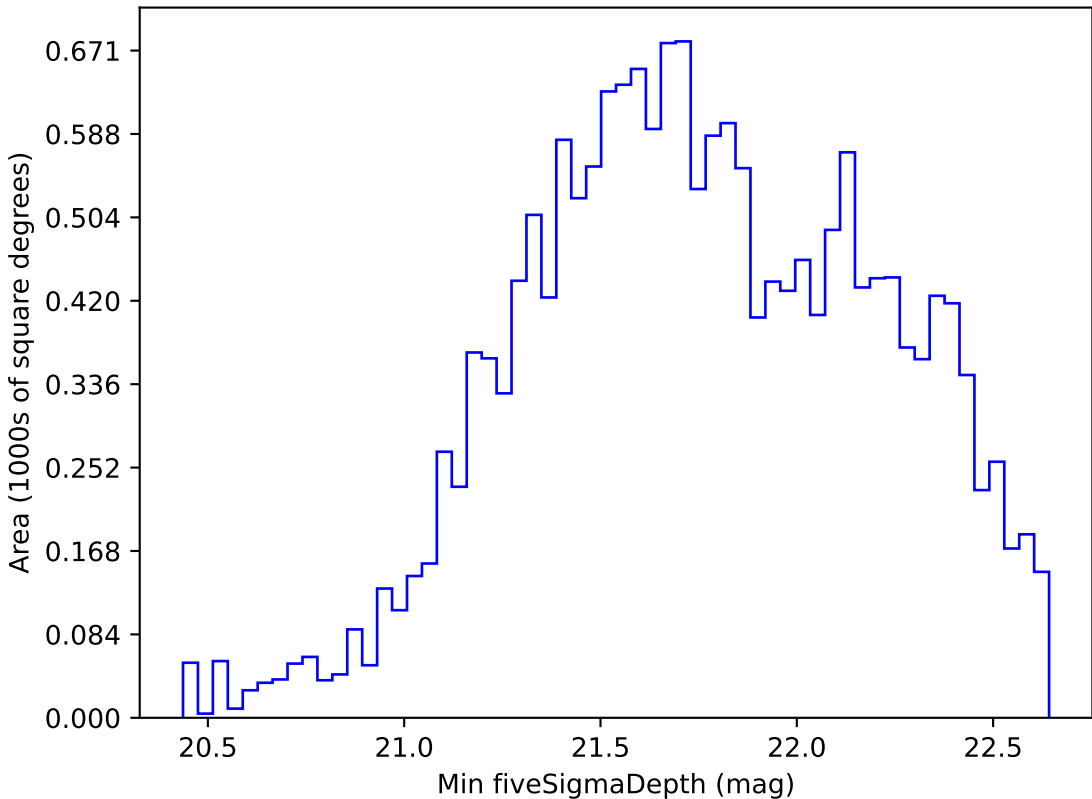
weather_cloudso0v3.5_10yrs WFD i band: Min fiveSigmaDepth
