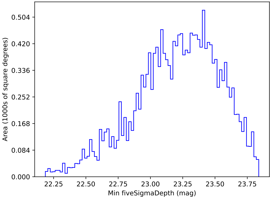
weather_cloudso0v3.5_10yrs WFD g band: Min fiveSigmaDepth
