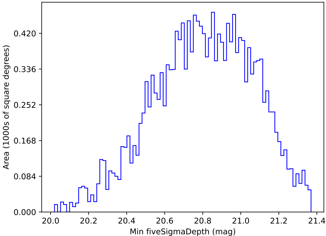
weather_cloudso0v3.5_10yrs WFD all bands: Min fiveSigmaDepth
