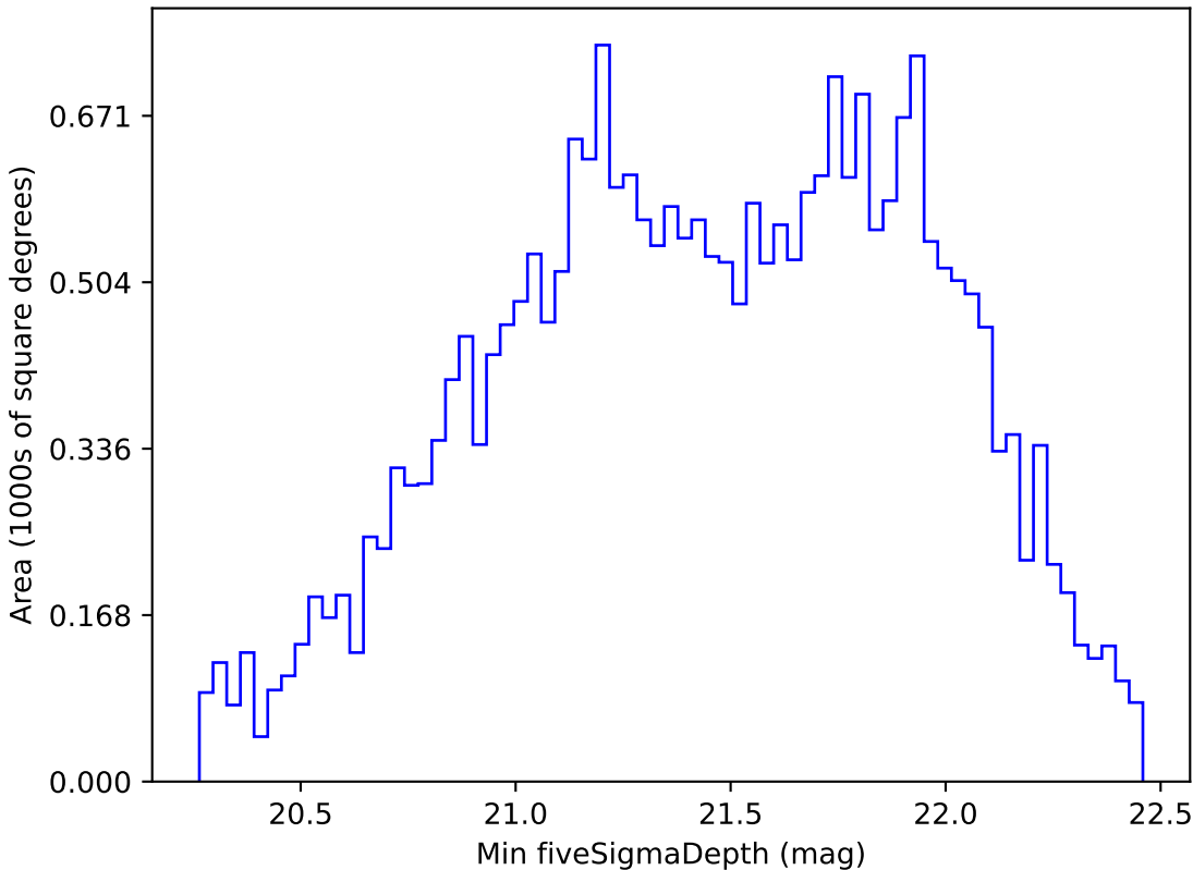
weather_cloudso0v3.5_10yrs All sky z band: Min fiveSigmaDepth
