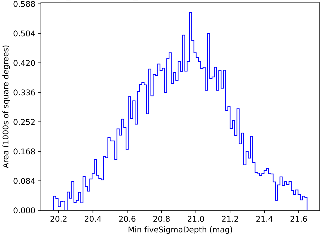
weather_cloudso0v3.5_10yrs All sky y band: Min fiveSigmaDepth
