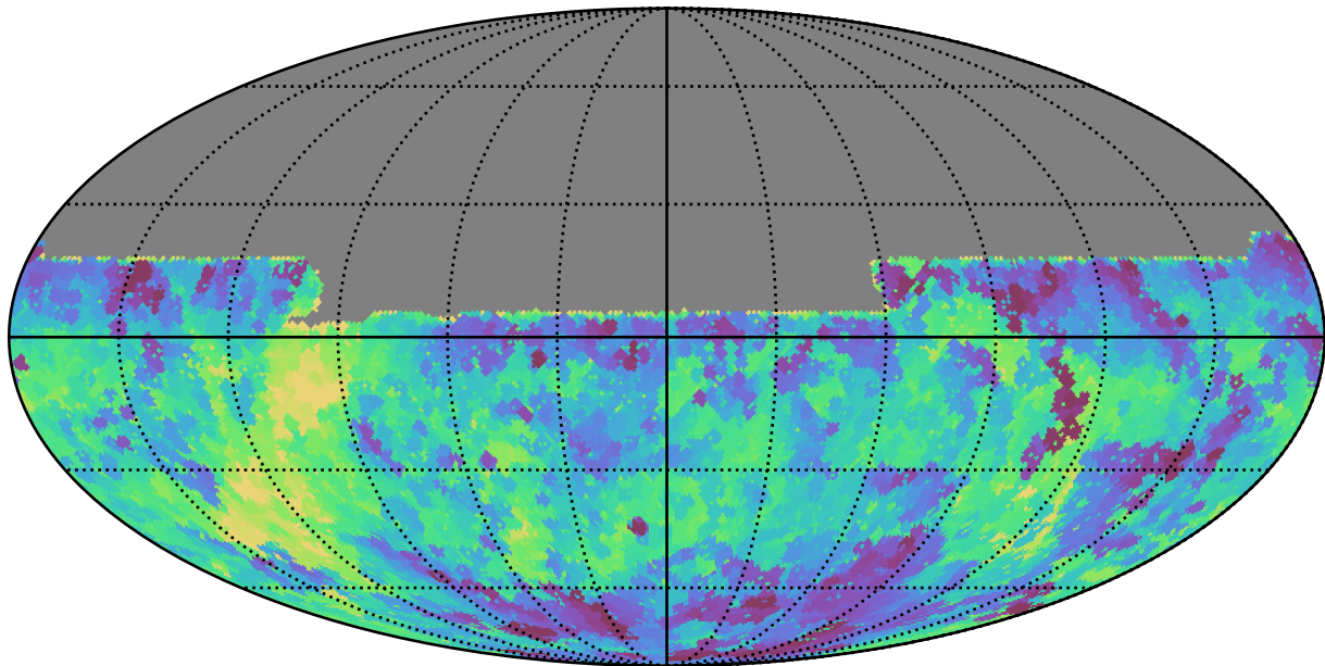
weather_cloudso0v3.5_10yrs All sky u band: Min fiveSigmaDepth
