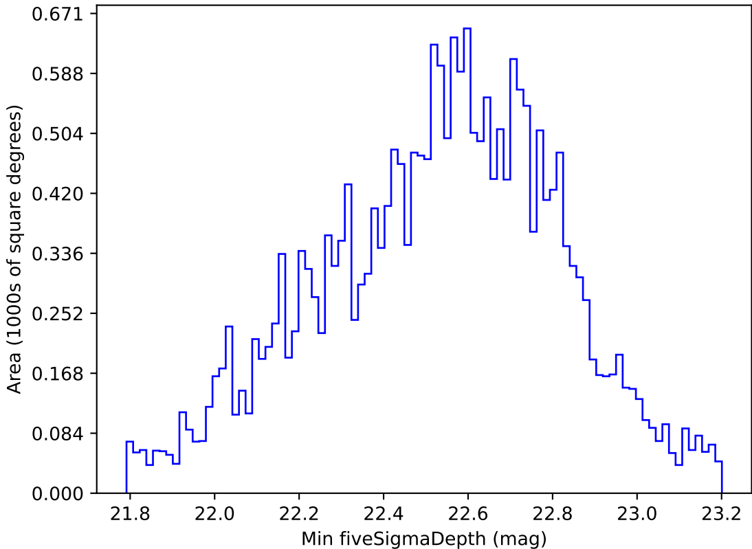
weather_cloudso0v3.5_10yrs All sky u band: Min fiveSigmaDepth
