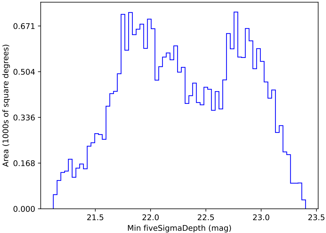
weather_cloudso0v3.5_10yrs All sky r band: Min fiveSigmaDepth
