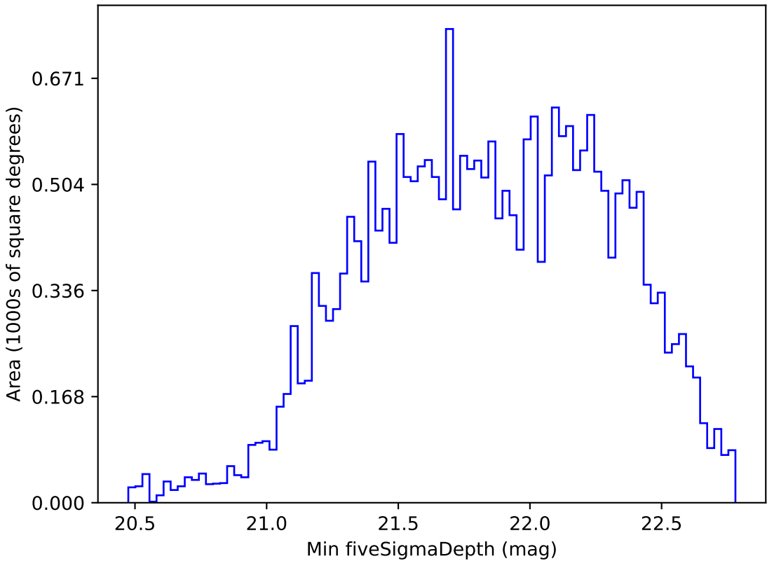
weather_cloudso0v3.5_10yrs All sky i band: Min fiveSigmaDepth
