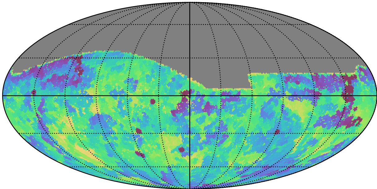
weather_cloudso0v3.5_10yrs All sky g band: Min fiveSigmaDepth
