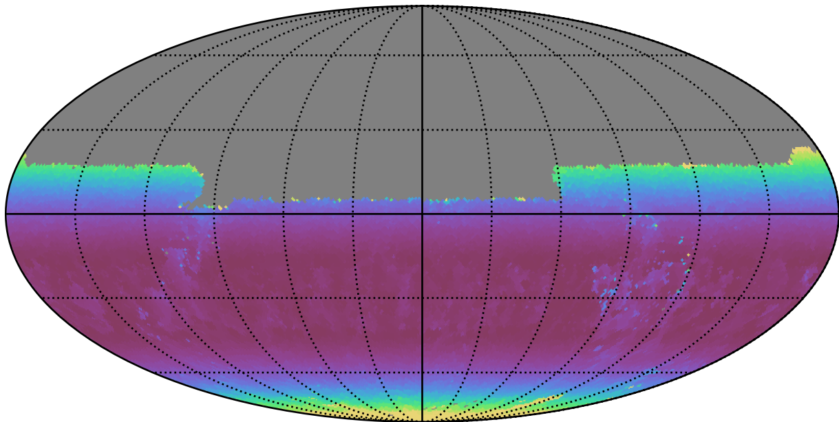
weather_cloudso0v3.5_10yrs Yr 1 y band: Min airmass
