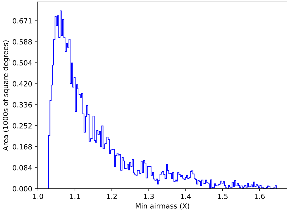
weather_cloudso0v3.5_10yrs Yr 1 u band: Min airmass
