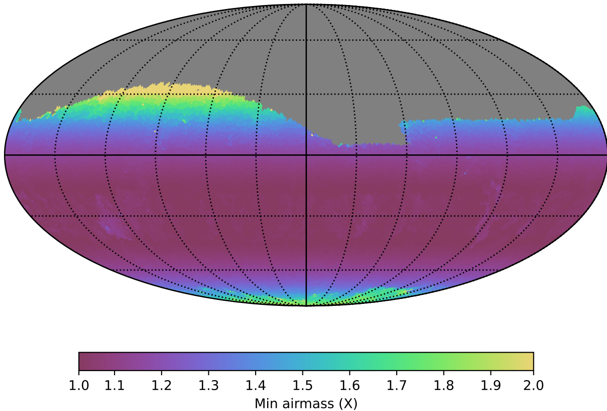
weather_cloudso0v3.5_10yrs Yr 1 i band: Min airmass
