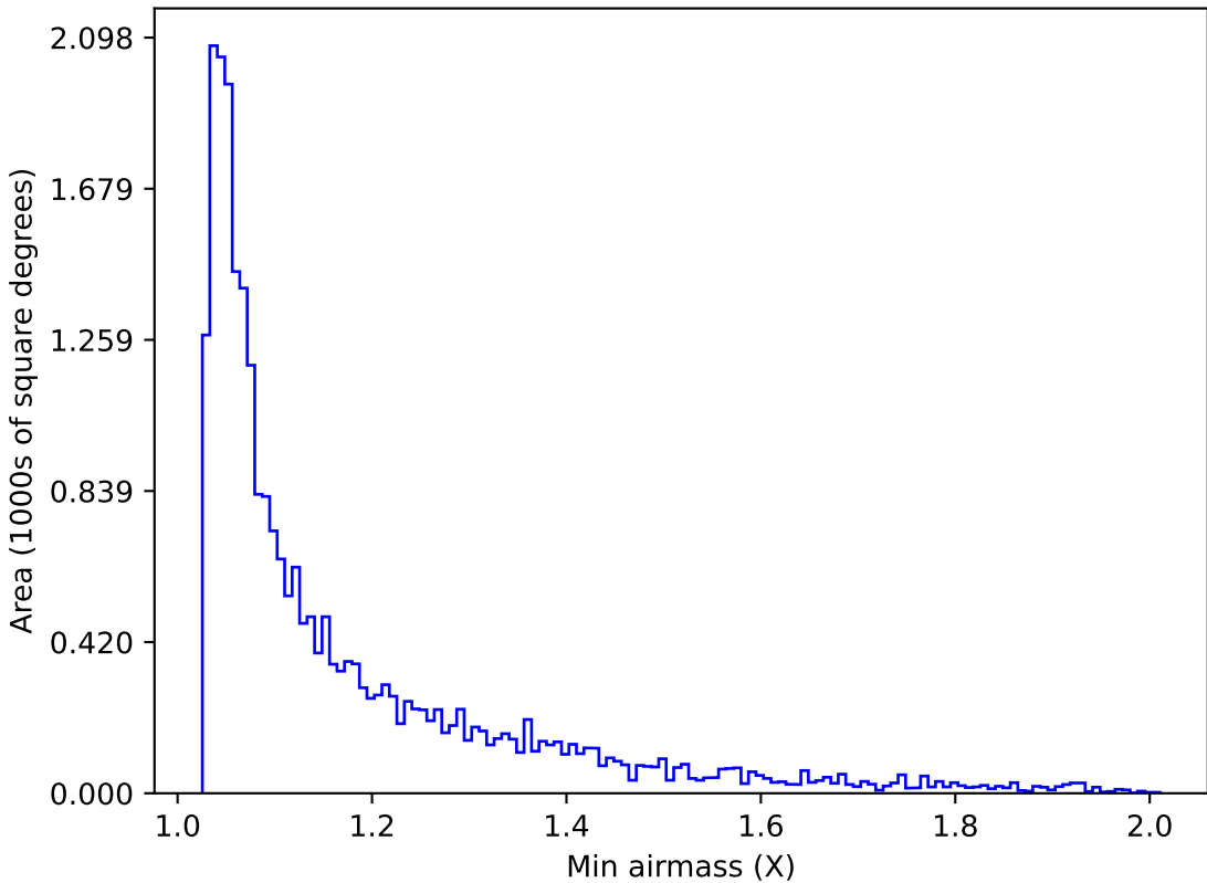
weather_cloudso0v3.5_10yrs Yr 1 g band: Min airmass
