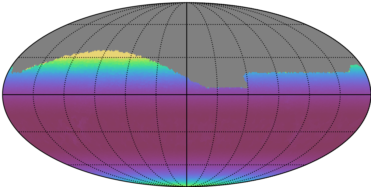
weather_cloudso0v3.5_10yrs Yr 1 all bands: Min airmass
