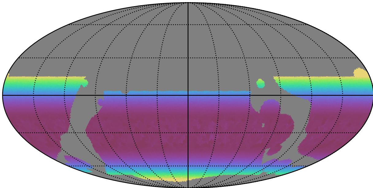
weather_cloudso0v3.5_10yrs WFD z band: Min airmass
