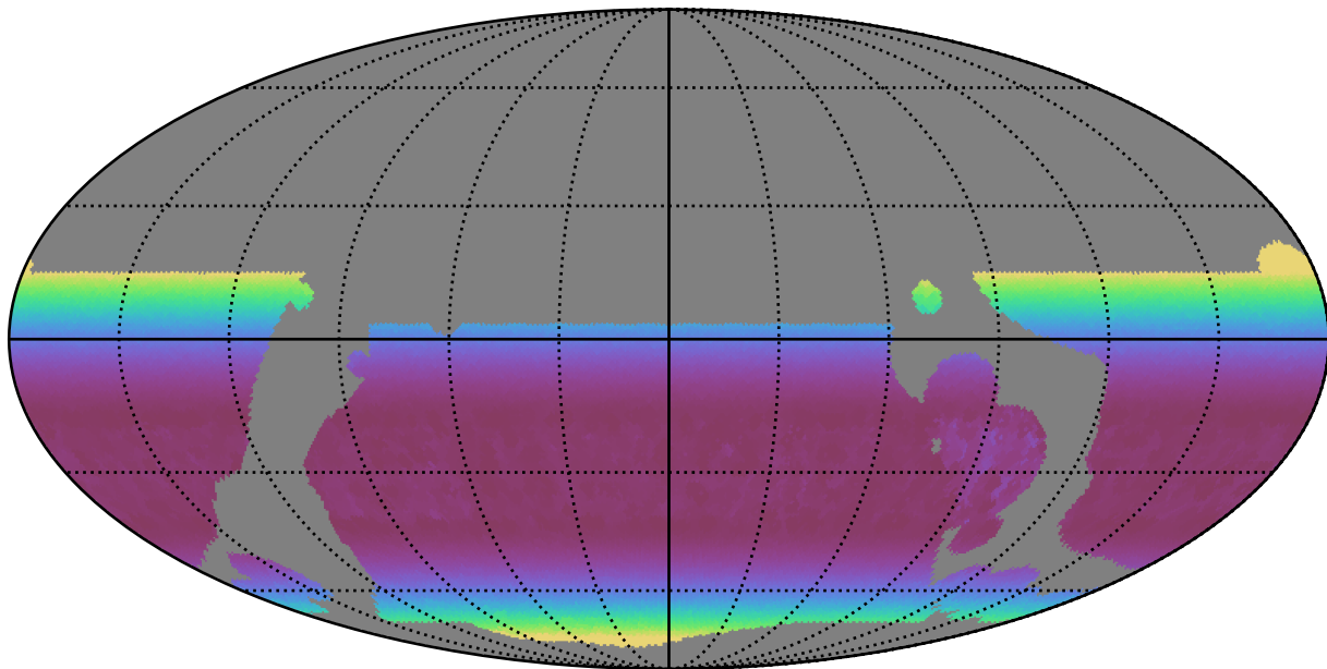
weather_cloudso0v3.5_10yrs WFD y band: Min airmass
