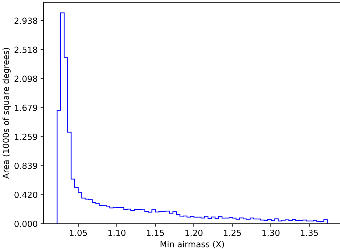
weather_cloudso0v3.5_10yrs WFD y band: Min airmass
