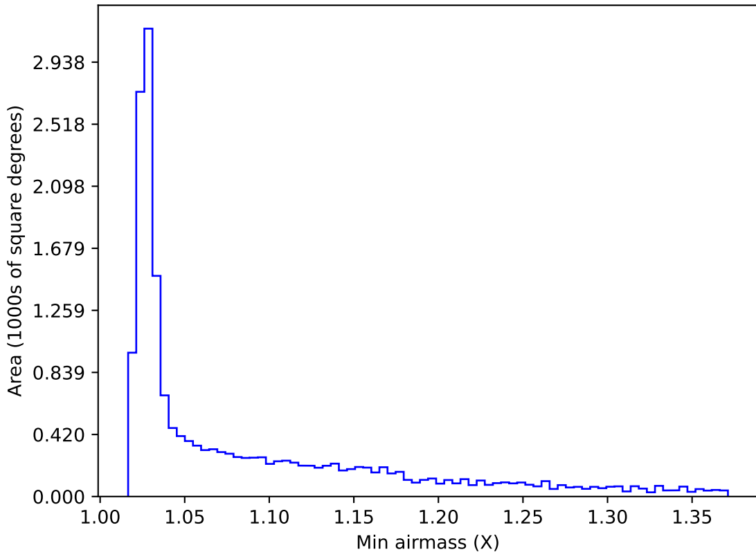
weather_cloudso0v3.5_10yrs WFD r band: Min airmass
