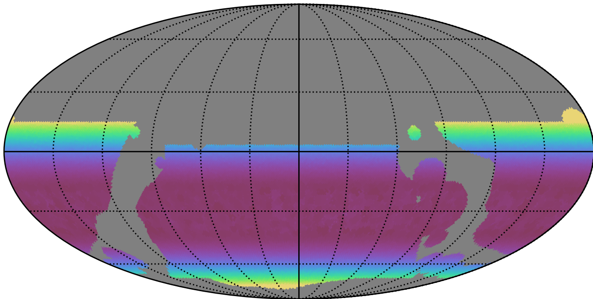
weather_cloudso0v3.5_10yrs WFD i band: Min airmass
