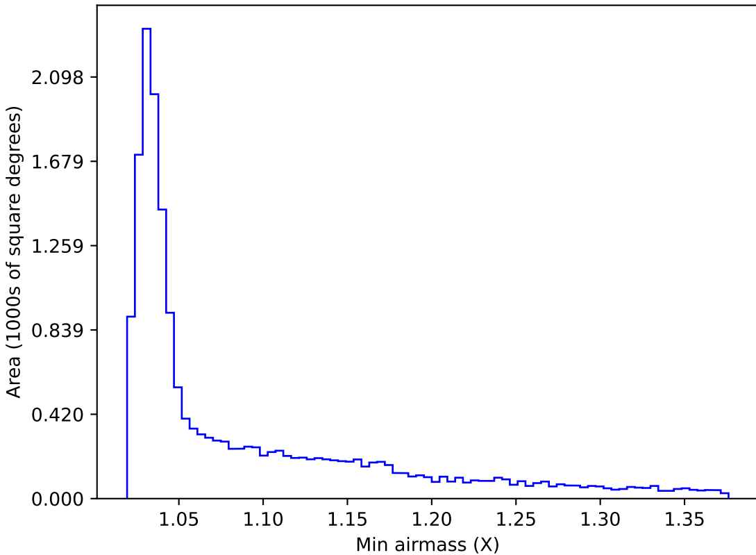
weather_cloudso0v3.5_10yrs WFD g band: Min airmass
