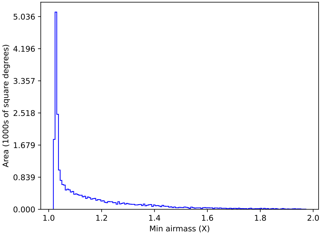
weather_cloudso0v3.5_10yrs All sky z band: Min airmass
