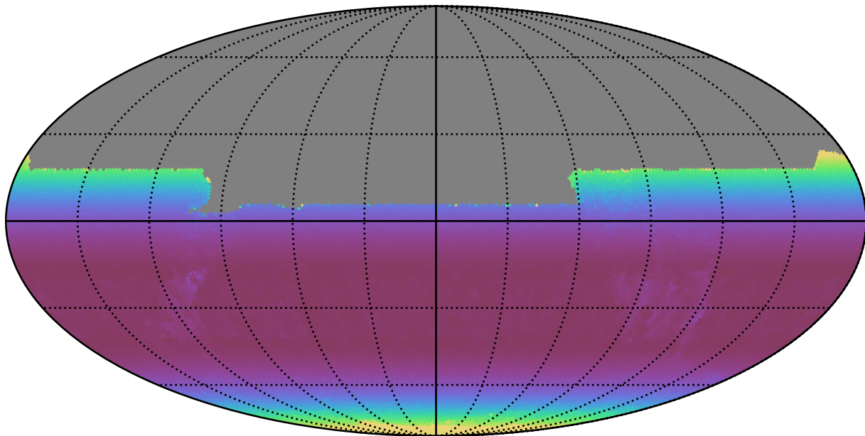
weather_cloudso0v3.5_10yrs All sky y band: Min airmass
