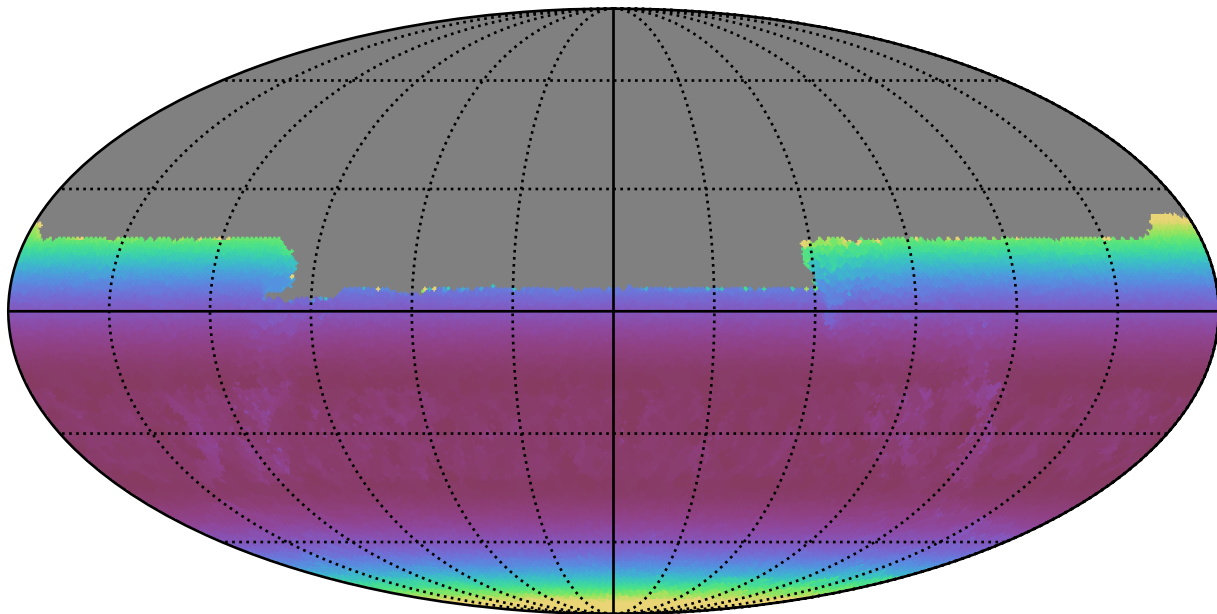
weather_cloudso0v3.5_10yrs All sky u band: Min airmass
