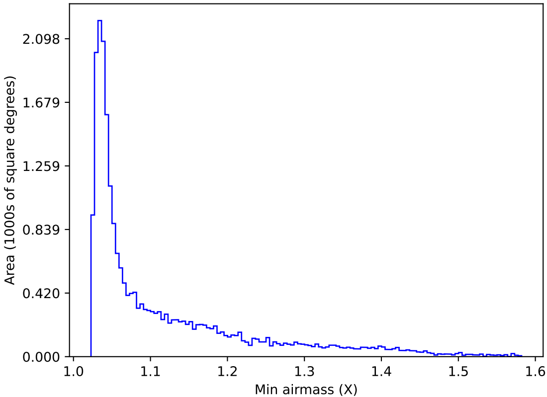
weather_cloudso0v3.5_10yrs All sky u band: Min airmass
