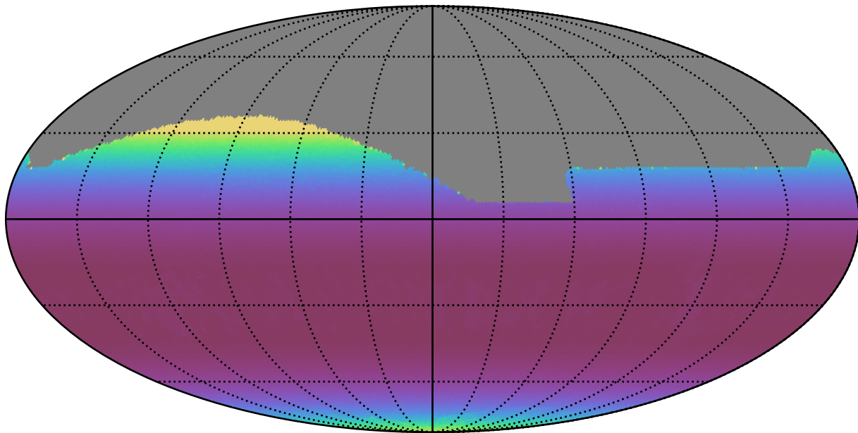
weather_cloudso0v3.5_10yrs All sky r band: Min airmass
