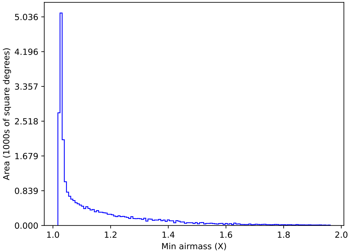
weather_cloudso0v3.5_10yrs All sky r band: Min airmass
