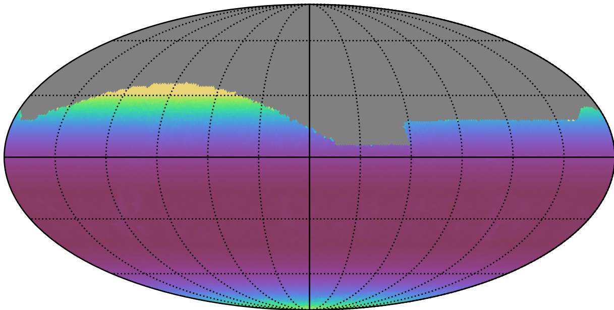
weather_cloudso0v3.5_10yrs All sky i band: Min airmass
