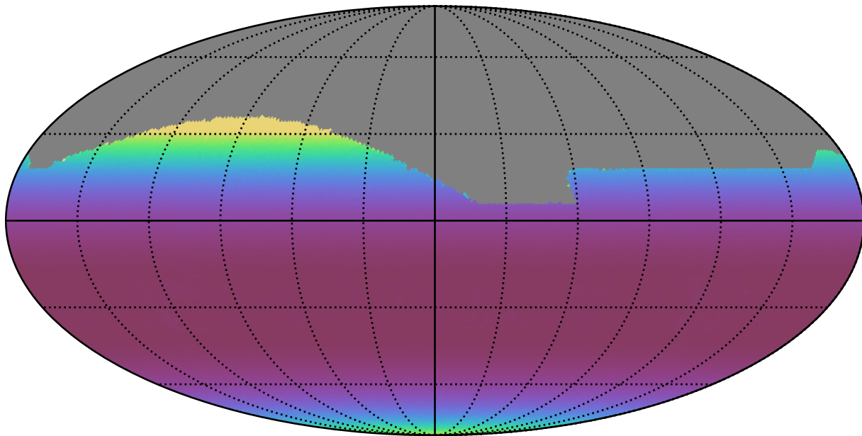
weather_cloudso0v3.5_10yrs All sky all bands: Min airmass
