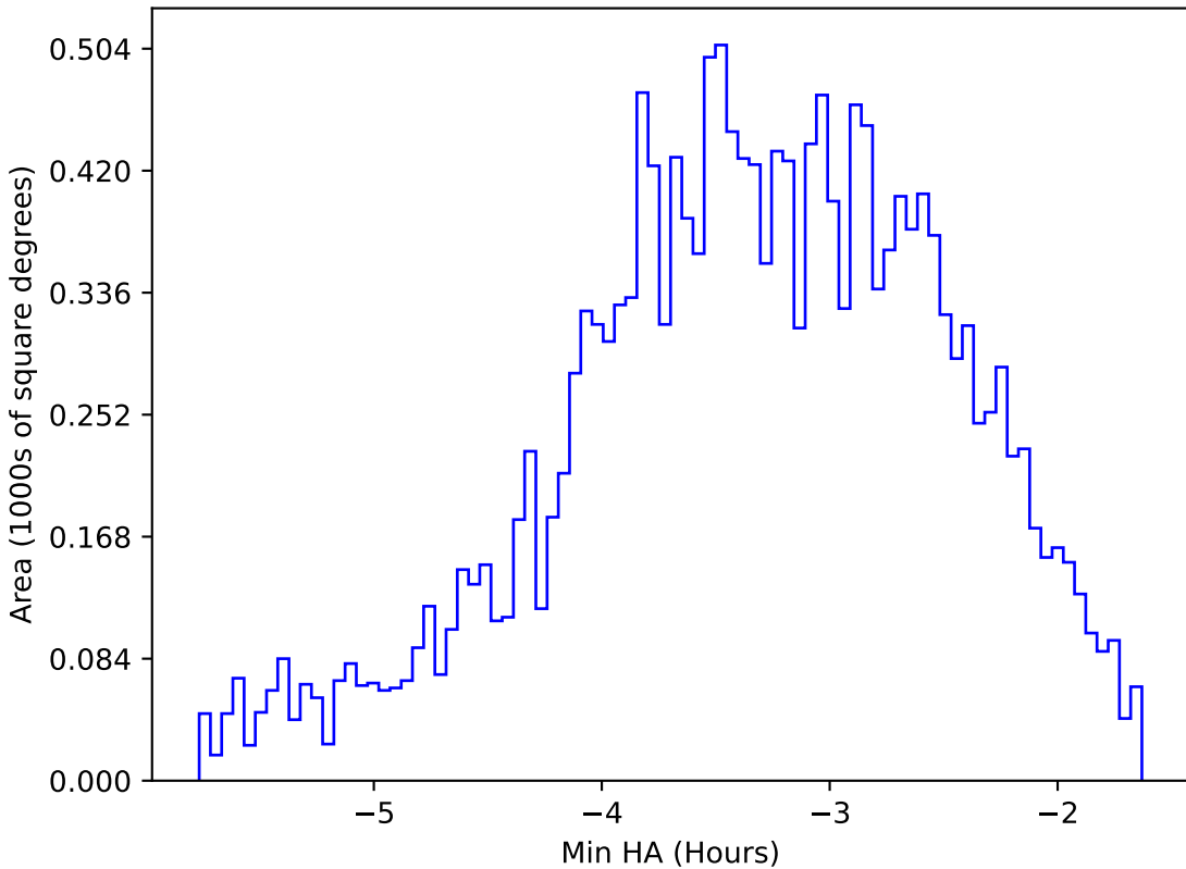
weather_cloudso0v3.5_10yrs WFD u band: Min HA
