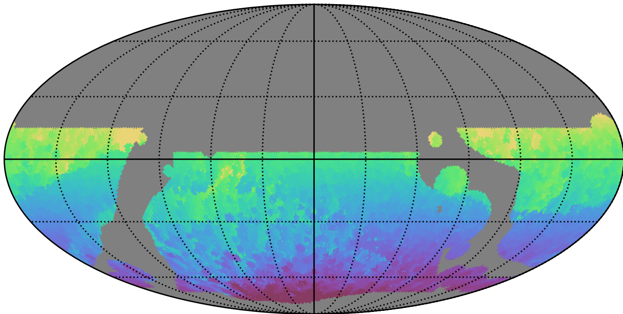
weather_cloudso0v3.5_10yrs WFD all bands: Min HA
