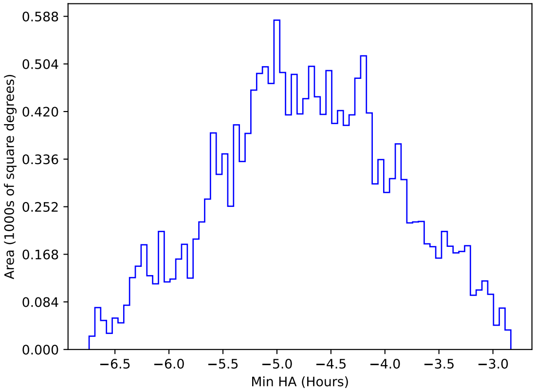
weather_cloudso0v3.5_10yrs WFD all bands: Min HA
