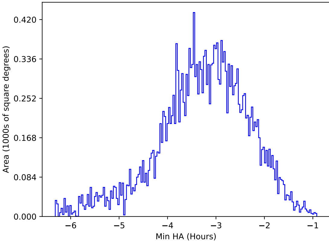
weather_cloudso0v3.5_10yrs All sky u band: Min HA
