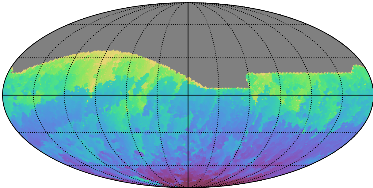
weather_cloudso0v3.5_10yrs All sky r band: Min HA
