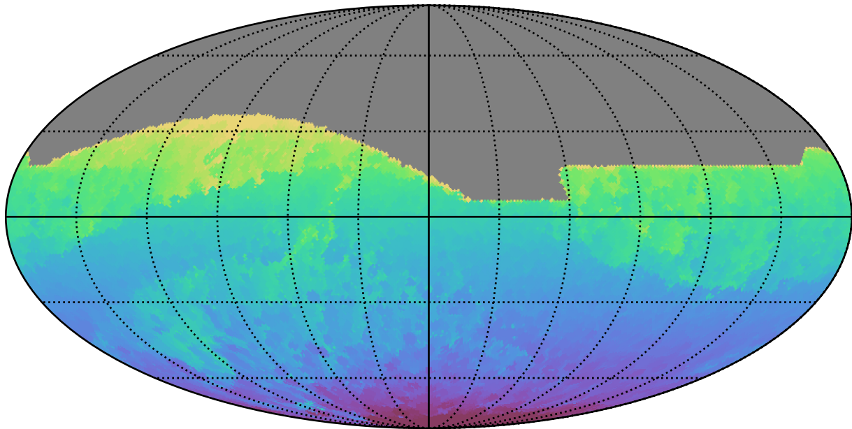
weather_cloudso0v3.5_10yrs All sky all bands: Min HA
