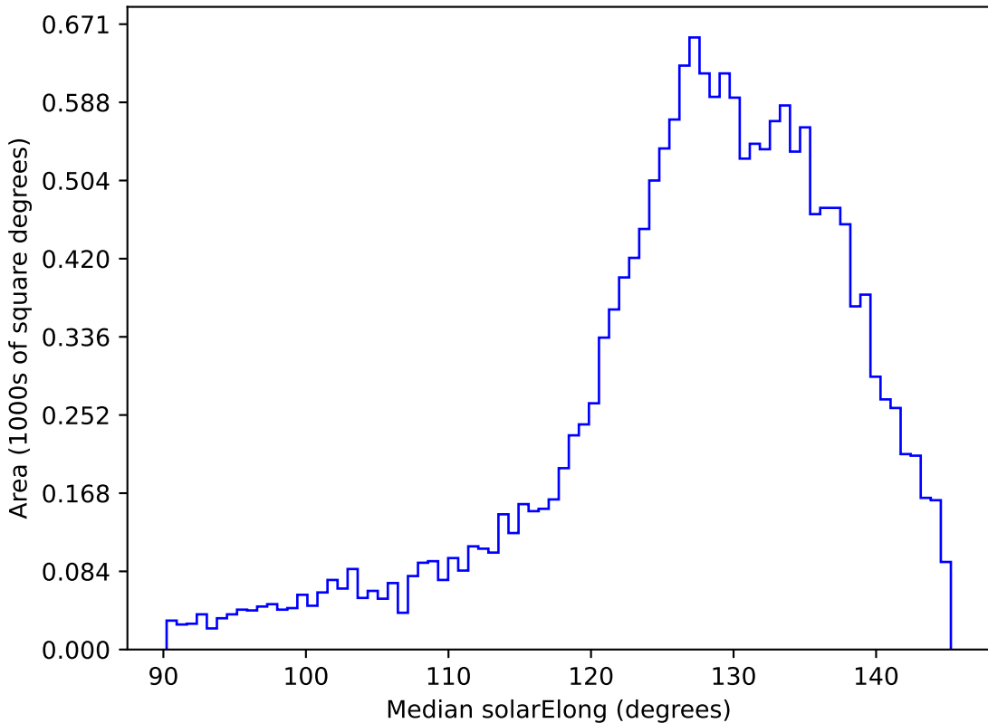
weather_cloudso0v3.5_10yrs WFD z band: Median solarElong
