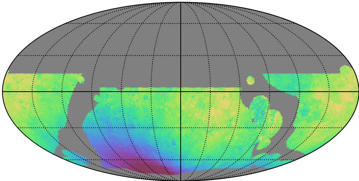
weather_cloudso0v3.5_10yrs WFD y band: Median solarElong
