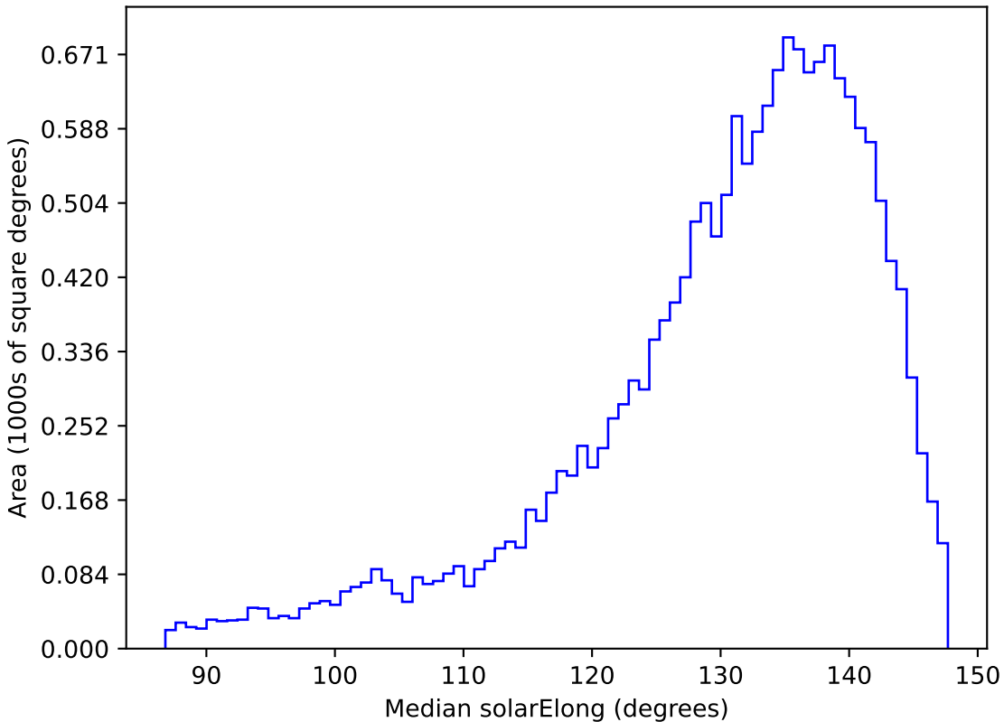
weather_cloudso0v3.5_10yrs WFD y band: Median solarElong
