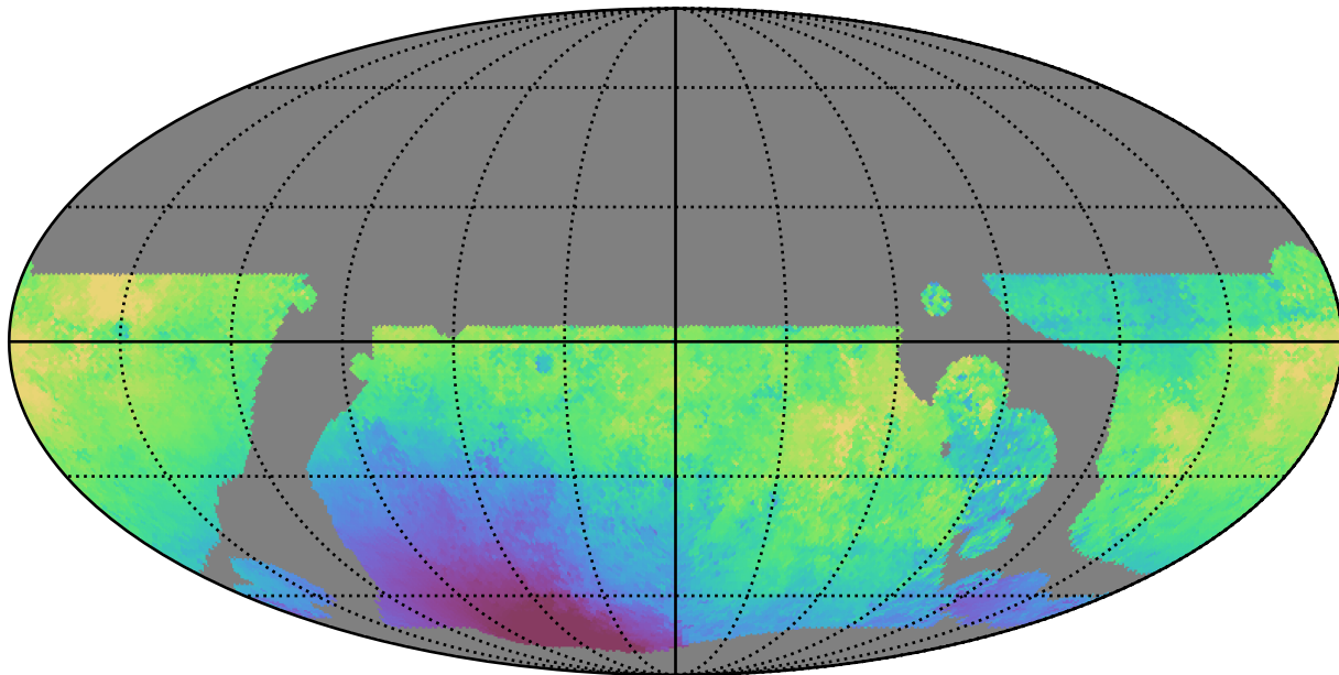
weather_cloudso0v3.5_10yrs WFD u band: Median solarElong
