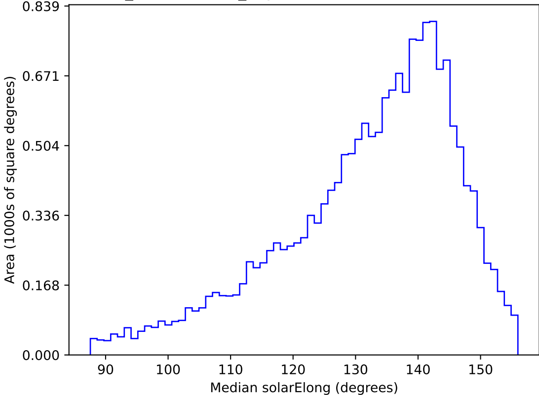
weather_cloudso0v3.5_10yrs WFD u band: Median solarElong
