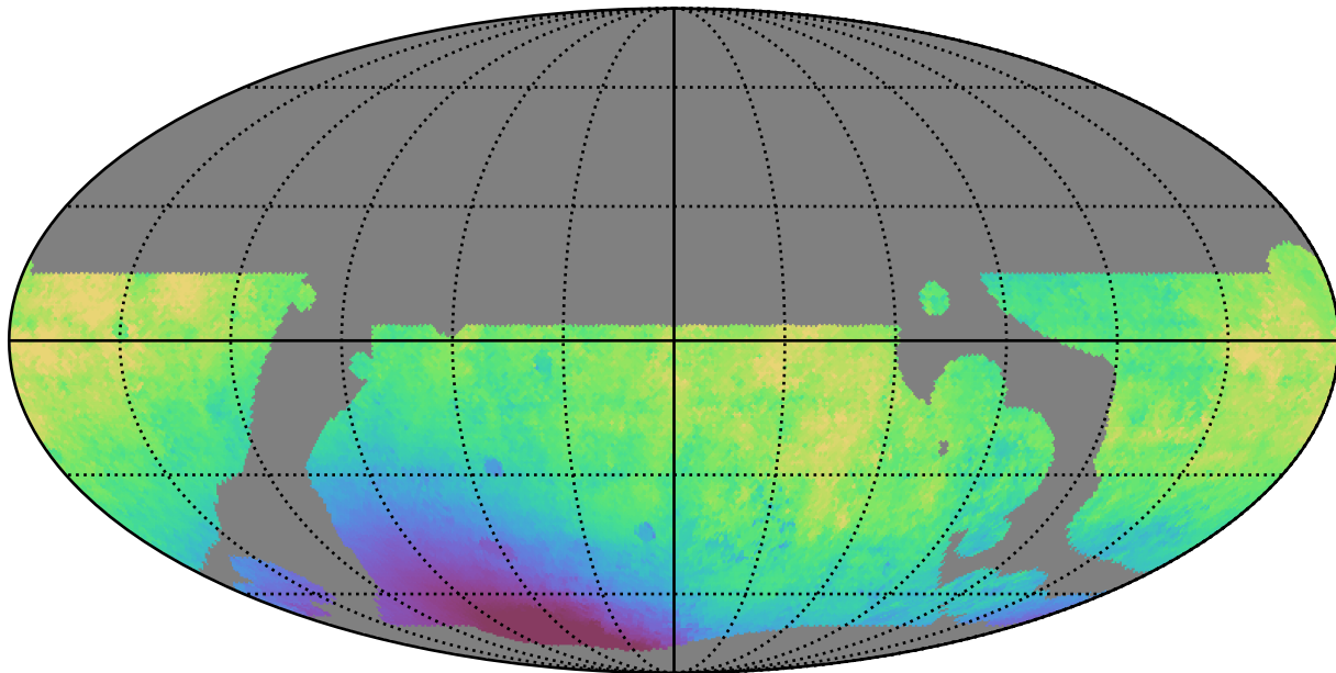
weather_cloudso0v3.5_10yrs WFD r band: Median solarElong
