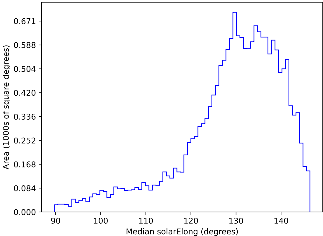
weather_cloudso0v3.5_10yrs WFD r band: Median solarElong
