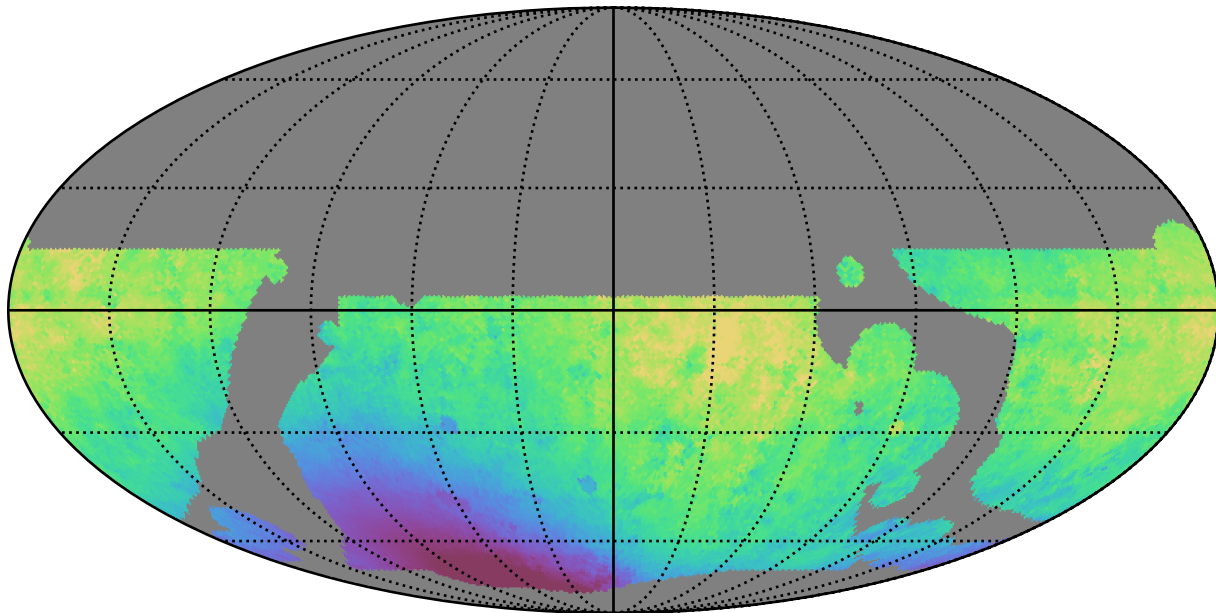
weather_cloudso0v3.5_10yrs WFD i band: Median solarElong
