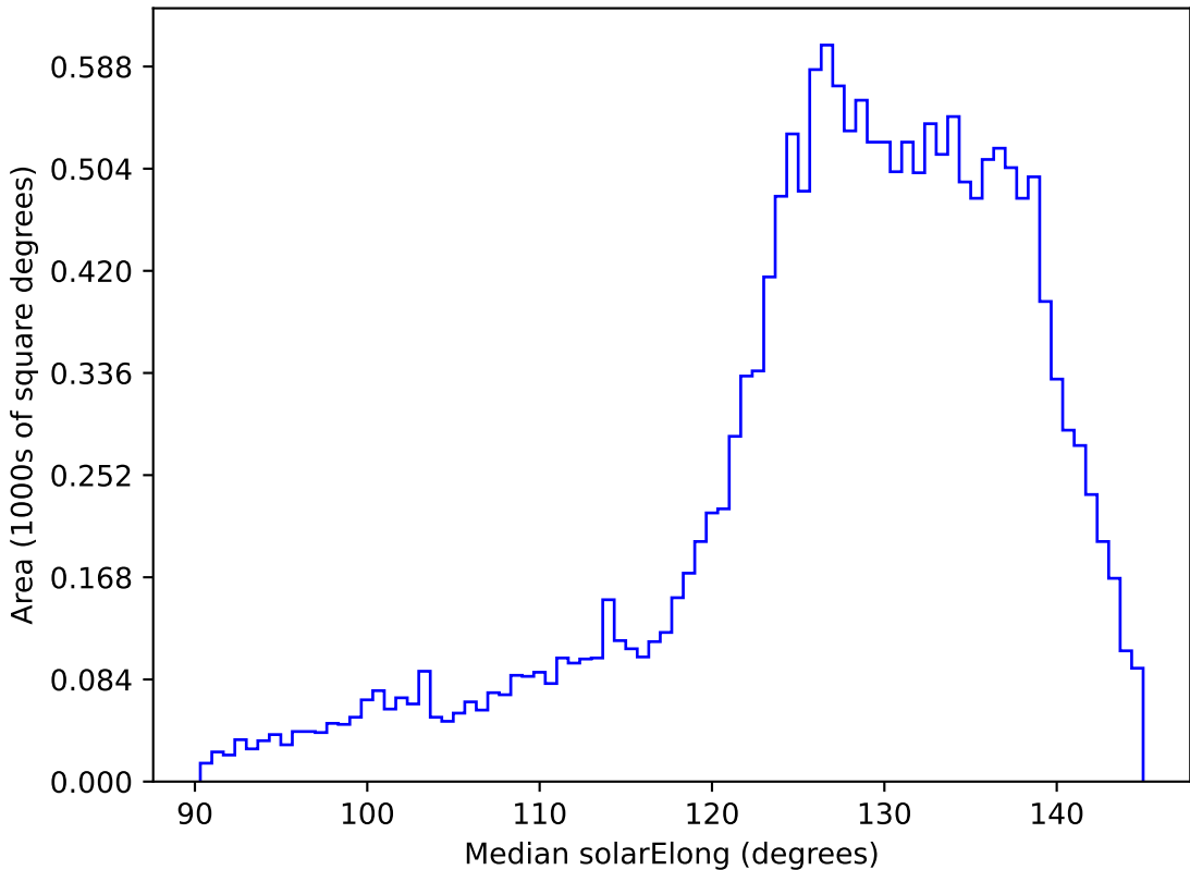
weather_cloudso0v3.5_10yrs WFD i band: Median solarElong
