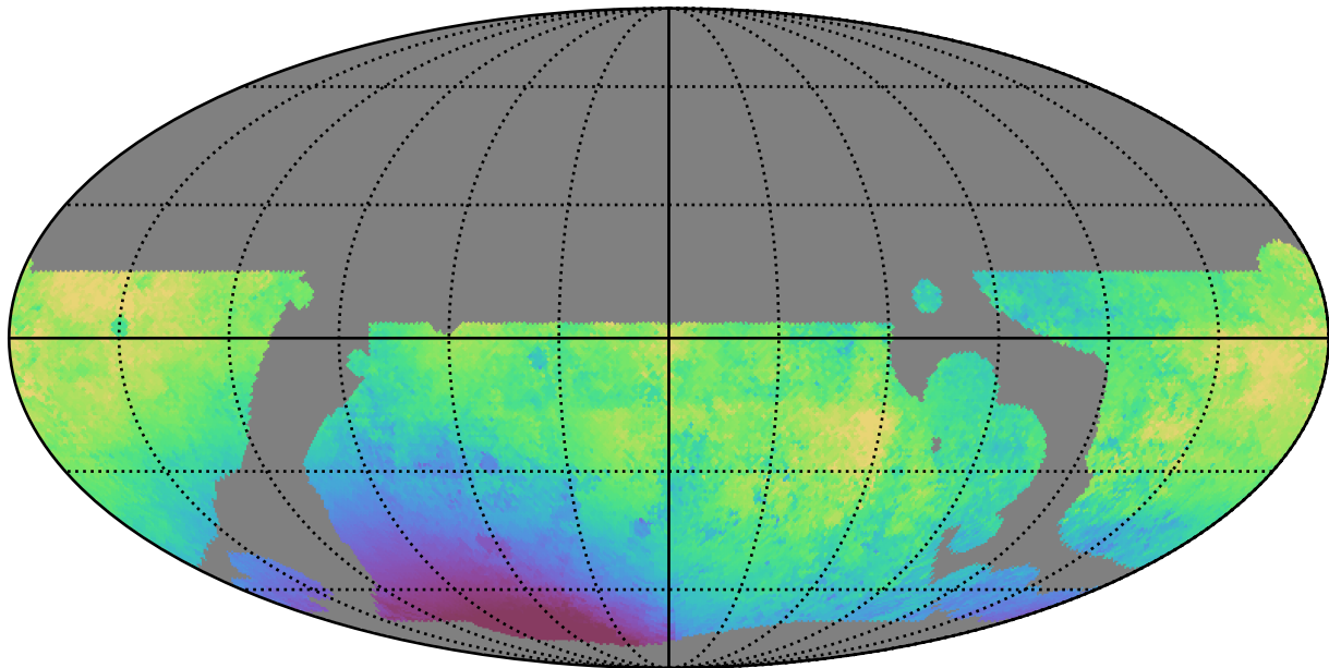
weather_cloudso0v3.5_10yrs WFD g band: Median solarElong
