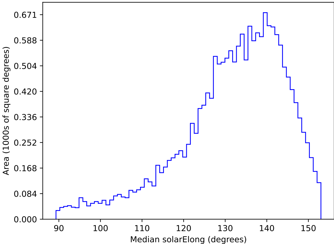
weather_cloudso0v3.5_10yrs WFD g band: Median solarElong
