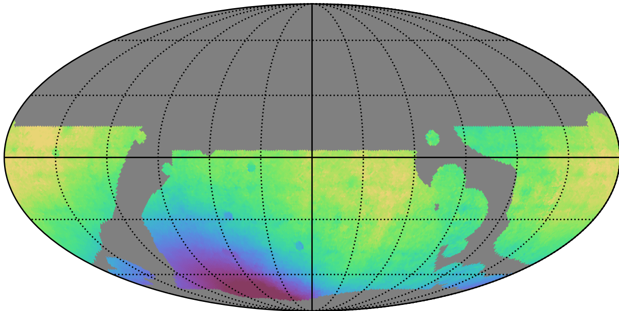
weather_cloudso0v3.5_10yrs WFD all bands: Median solarElong
