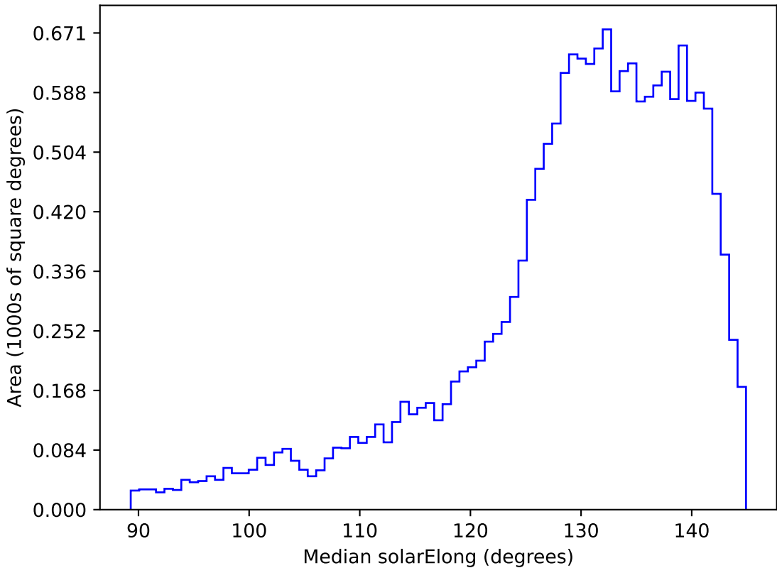
weather_cloudso0v3.5_10yrs WFD all bands: Median solarElong
