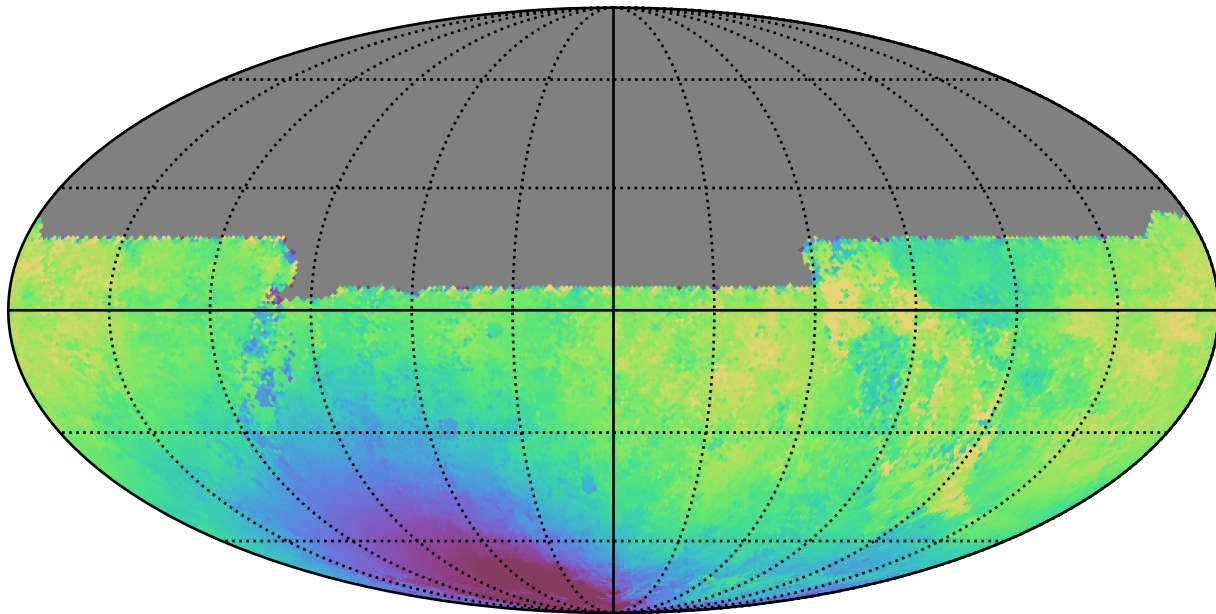
weather_cloudso0v3.5_10yrs All sky y band: Median solarElong
