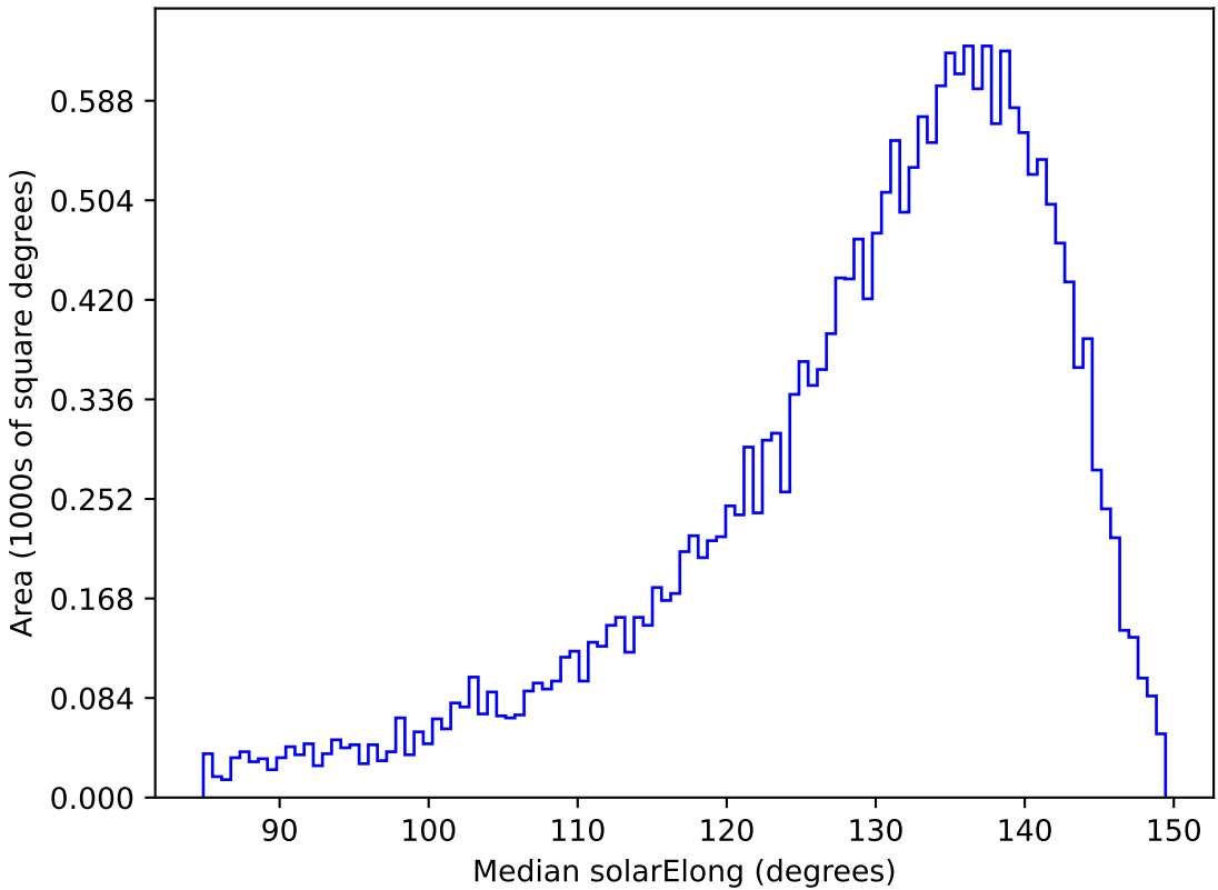
weather_cloudso0v3.5_10yrs All sky y band: Median solarElong
